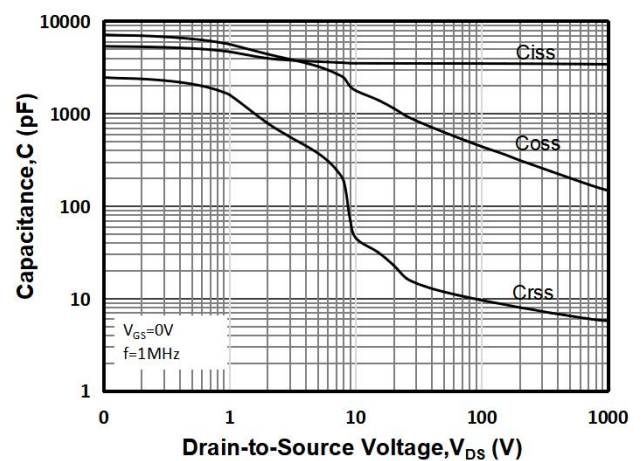
Fig 12: Capacitance Characteristics
