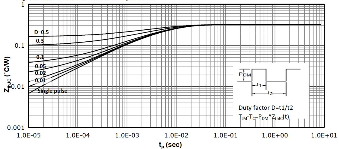
Fig 13: Max. Transient Thermal Impedance
