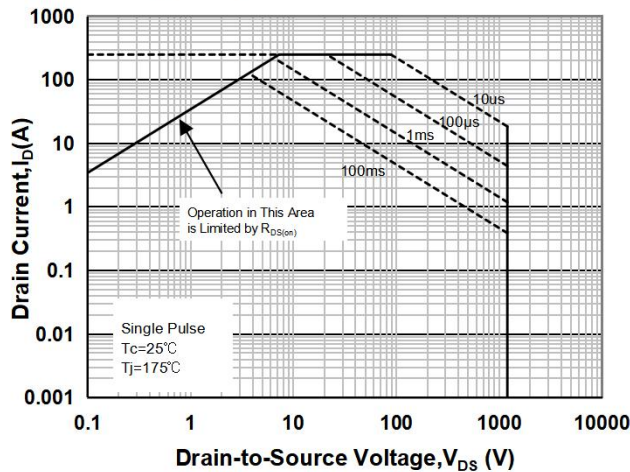
Fig 15: Safe Operating Area
