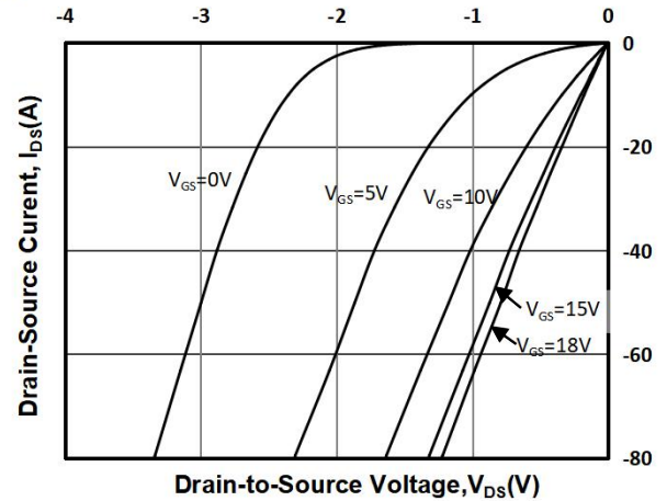
Fig 10: 3rd Quadrant Characteristic at 25°C
