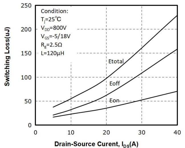
Fig 21: I_{DS}(\text{A}) vs. Switching Loss(uJ)
