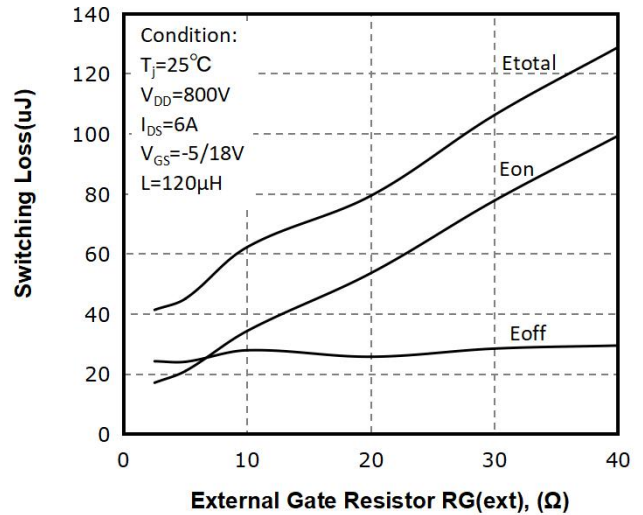
Fig 19: R_g(\Omega) vs. Switching Loss(uJ)
