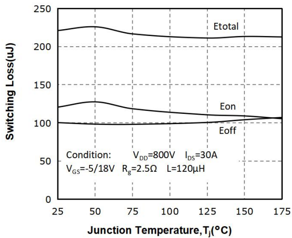
Fig 20: Temperature( ^\circ\text{C} ) vs. Switching Loss(uJ)
