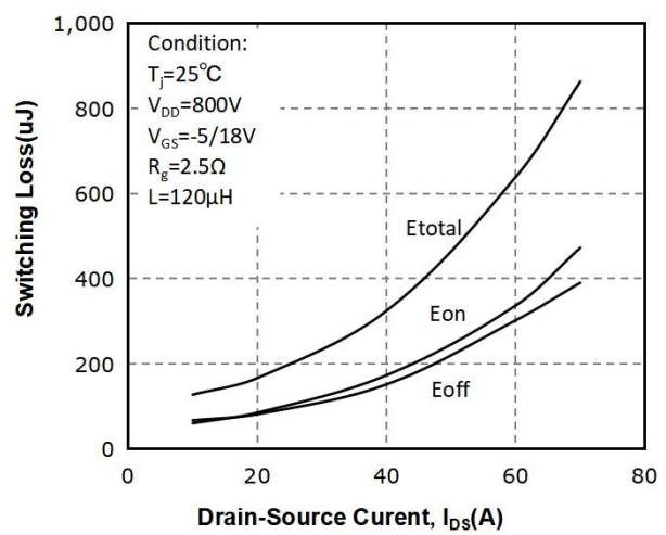
Fig 21: I_{DS}(\text{A}) vs. Switching Loss(uJ)
