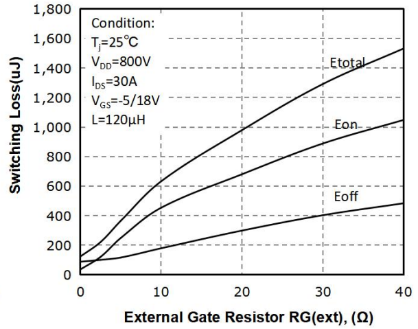
Fig 19: R_g(\Omega) vs. Switching Loss(uJ)
