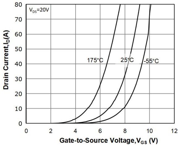
Fig 7: Transfer Characteristics
