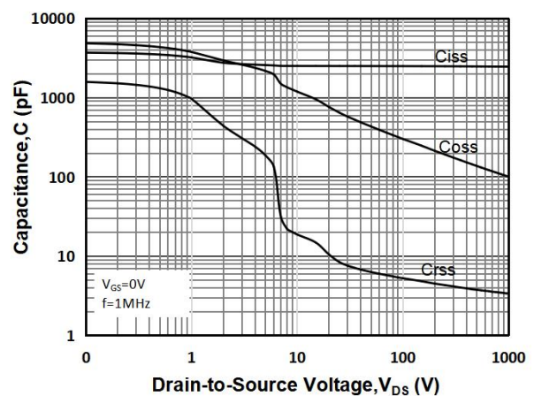
Fig 12: Capacitance Characteristics
