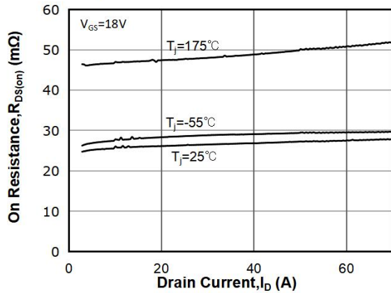
Fig 5: On-Resistance vs. Drain Current For Various Temperatures
