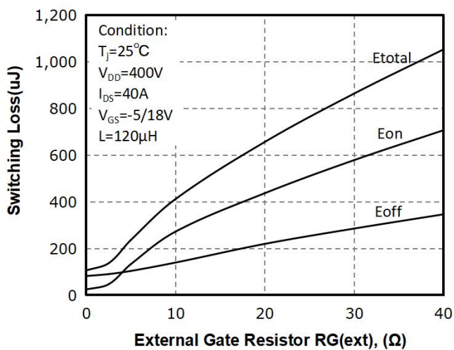
Fig 19: R_g(\Omega) vs. Switching Loss(uJ)
