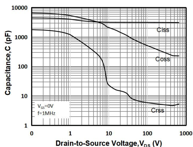
Fig 12: Capacitance Characteristics
