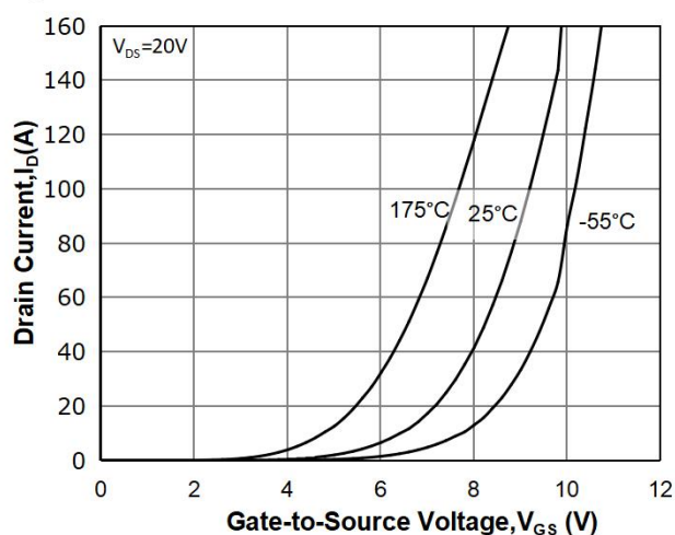
Fig 7: Transfer Characteristics
