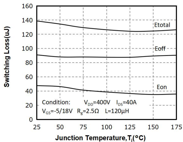
Fig 20: Temperature( ^\circ\text{C} ) vs. Switching Loss(uJ)
