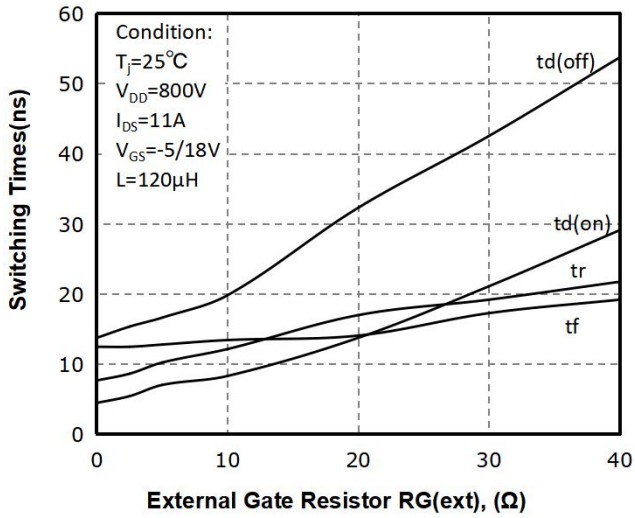
Fig 18: R_g(\Omega) vs. Switching Times(us)
