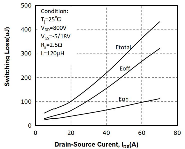
Fig 21: I_{DS}(\text{A}) vs. Switching Loss(uJ)
