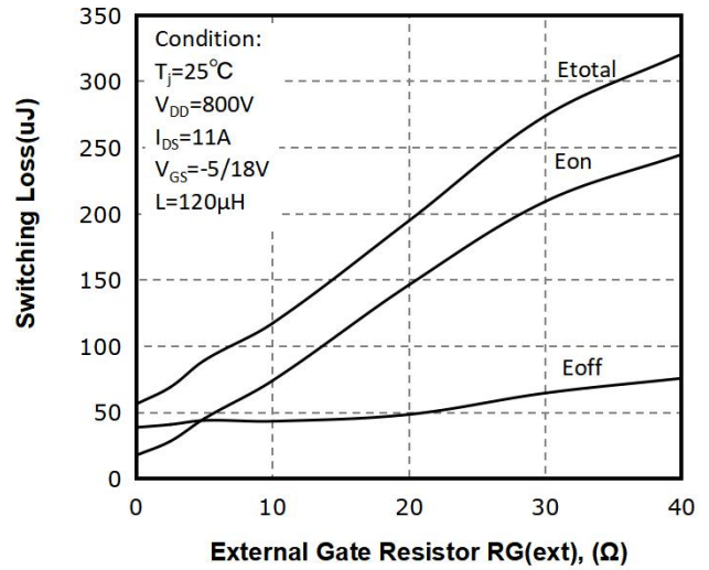
Fig 19: R_g(\Omega) vs. Switching Loss(uJ)
