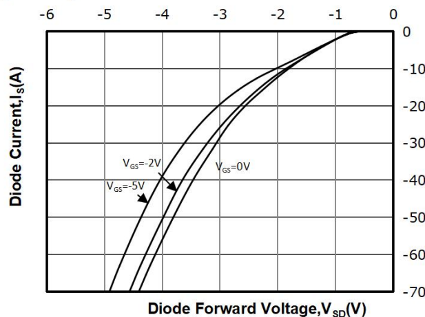
Fig 10: Body Diode Characteristic at 175°C
