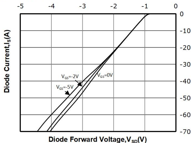
Fig 8: Body Diode Characteristic at 25°C
