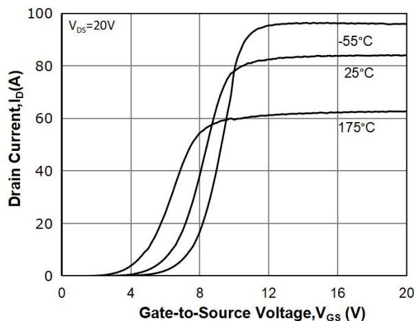
Fig 7: Transfer Characteristics
