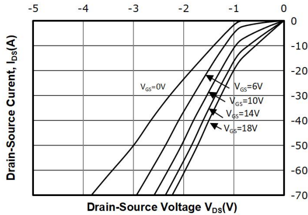
Fig 13: 3rd Quadrant Characteristic at 25°C
