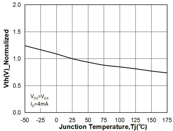
Fig 9: V_{th}(V) Vs T_j Characteristics
