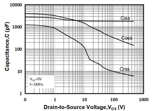
Fig 12: Capacitance Characteristics
