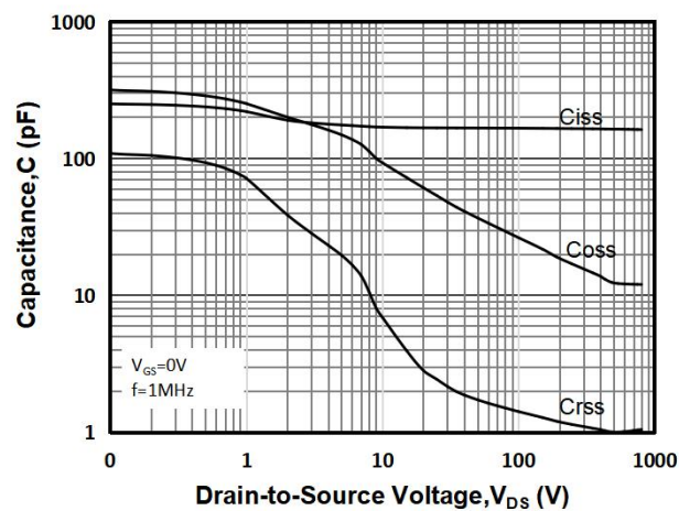
Fig 12: Capacitance Characteristics
