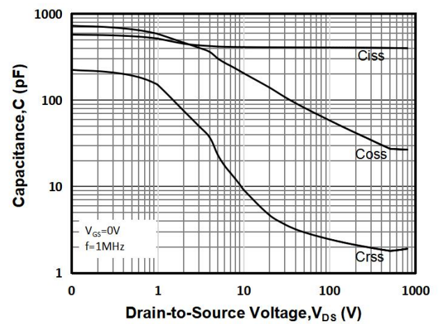
Fig 12: Capacitance Characteristics
