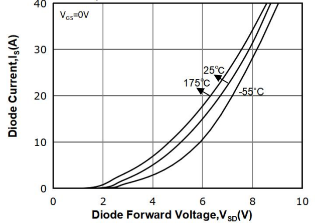
Fig 8: Body-diode Forward Characteristics For Various Temperatures
