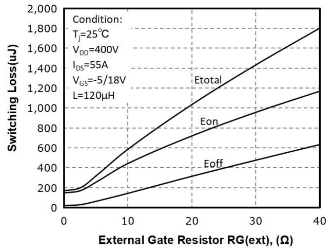
Fig 19: R_g(\Omega) vs. Switching Loss( \mu\text{J} )
