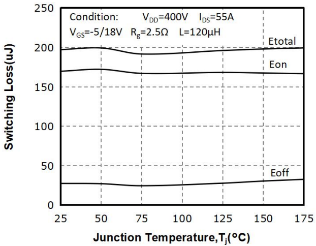
Fig 20: Temperature( ^\circ\text{C} ) vs. Switching Loss( \mu\text{J} )
