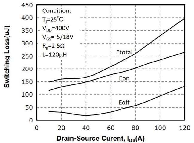
Fig 21: I_{DS}(\text{A}) vs. Switching Loss( \mu\text{J} )
