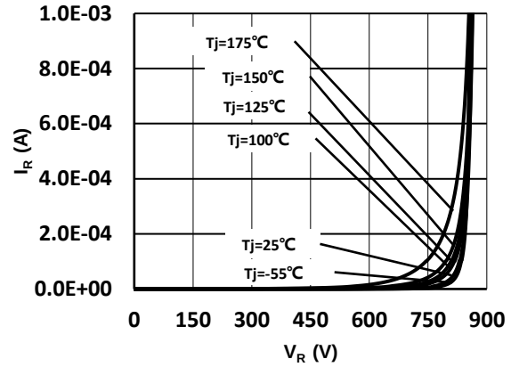
Fig 2: Reverse Characteristics
