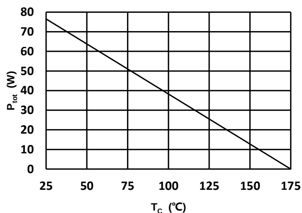
Fig 4: Power Derating
