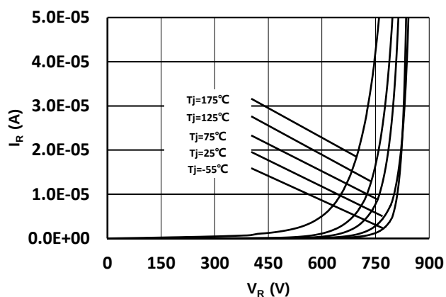
Fig 2: Reverse Characteristics
