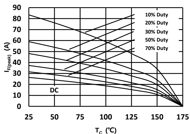
Fig 3: Current Derating
