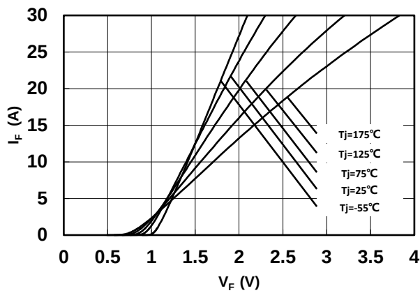
Fig 1: Forward Characteristics
