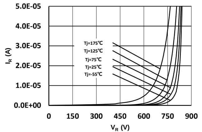
Fig 2: Reverse Characteristics
