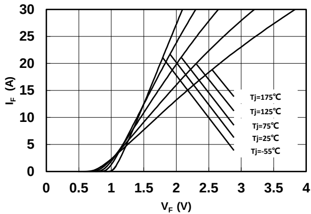
Fig 1: Forward Characteristics
